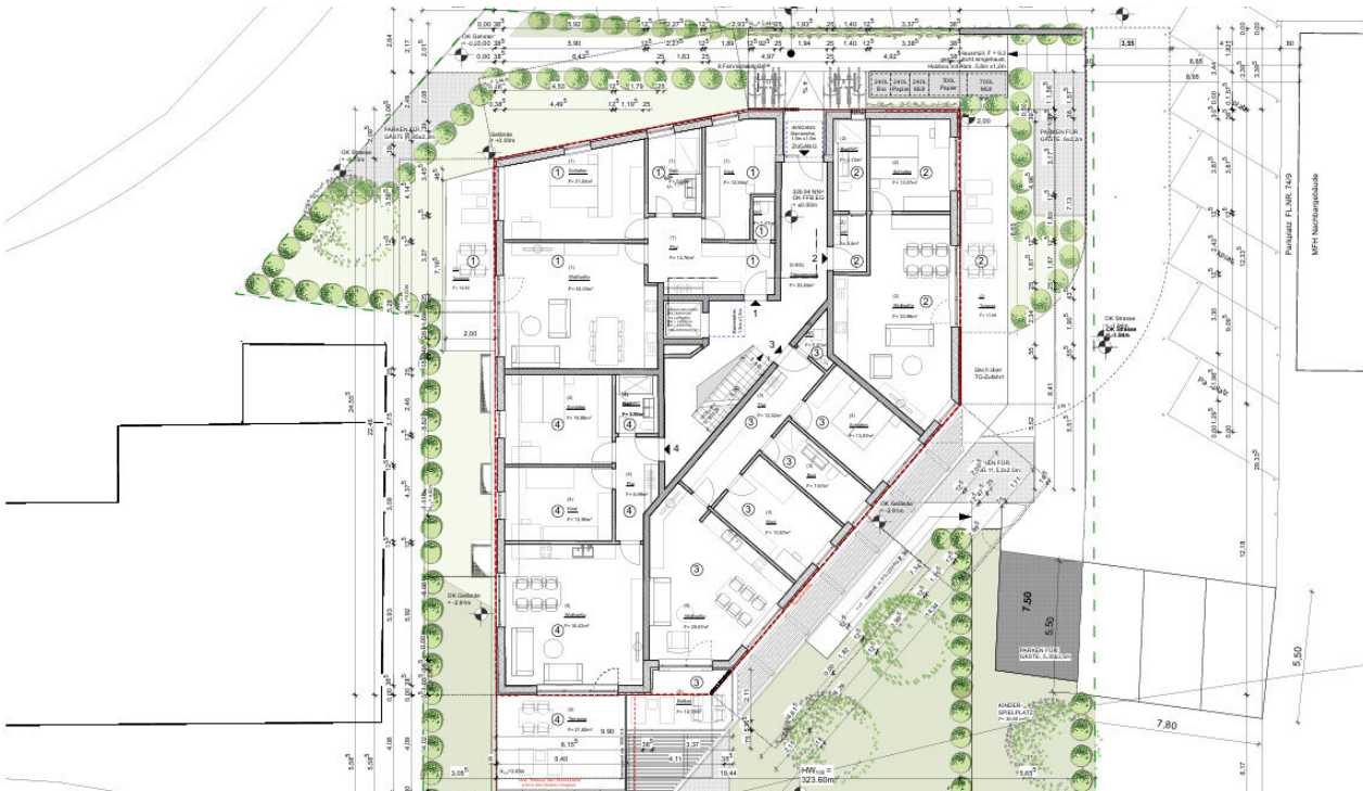
Grundriss EG Whg 1-4
