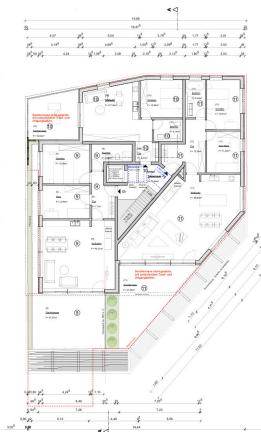
Grundriss DG Whg 9-11
